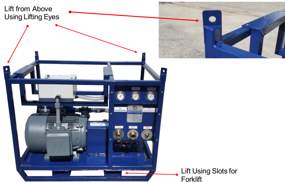
Figure 4.1 – Lifting Guidelines
