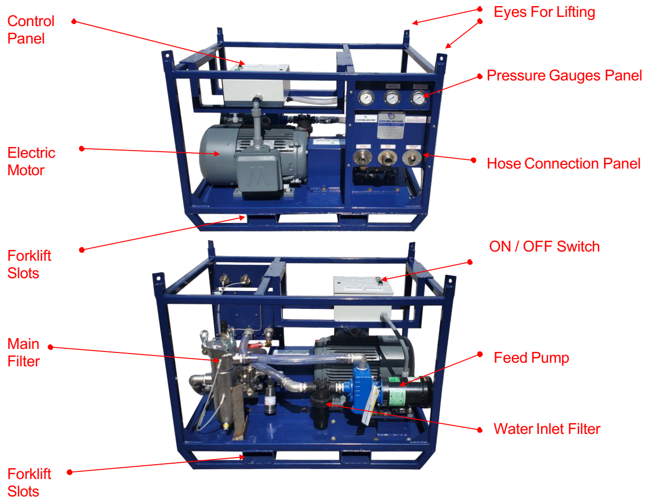
Figure 2.1 – CaviBlaster 1440-E General Features
