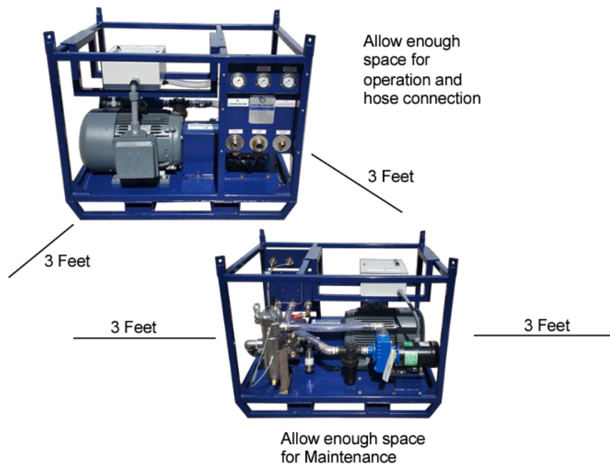
Figure 4.2 – Installation Guidelines
