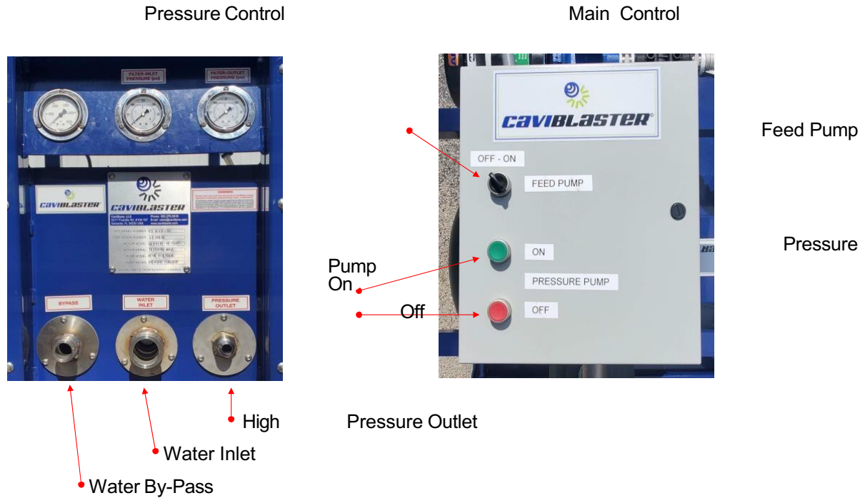
Figure 2.2 – CaviBlaster 1440-E Control Panel
