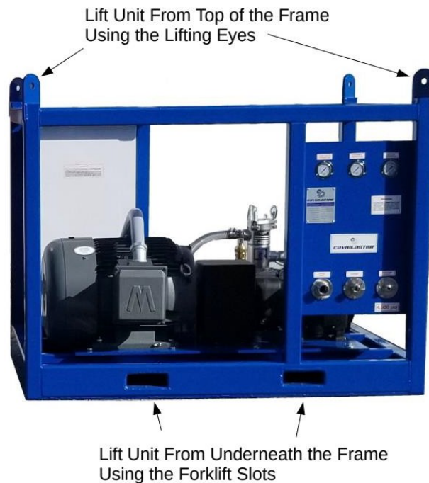
Figure 4.1 – Lifting Guidelines
