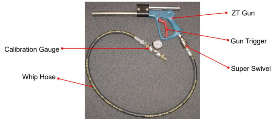
Figure 5.2 – Zero-thrust gun Pressure Calibration
