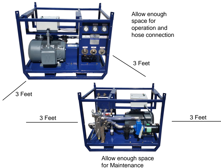
Figure 4.2 – Installation Guidelines
