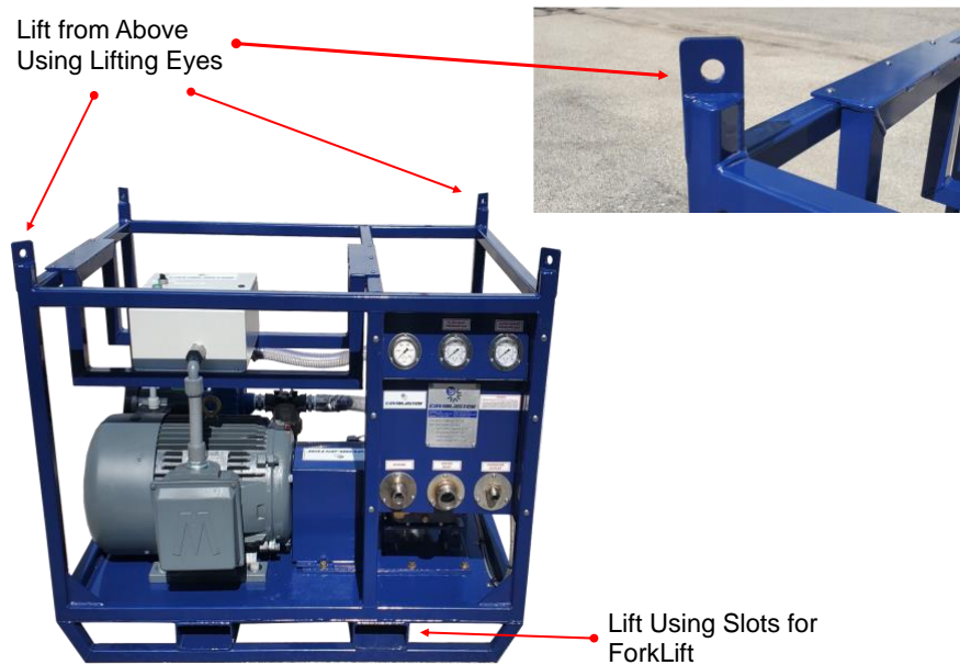
Figure 4.1 – Lifting Guidelines
