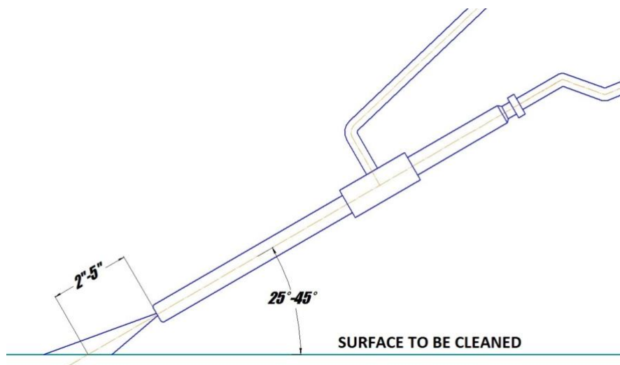
Figure 5.3 – Lance Position for Best Cleaning Results
